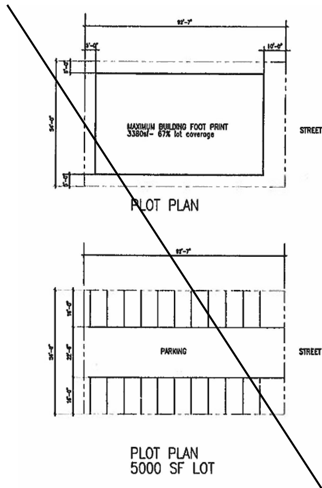
Figure 32-2.6 5,000 SQUARE FOOT LOT
