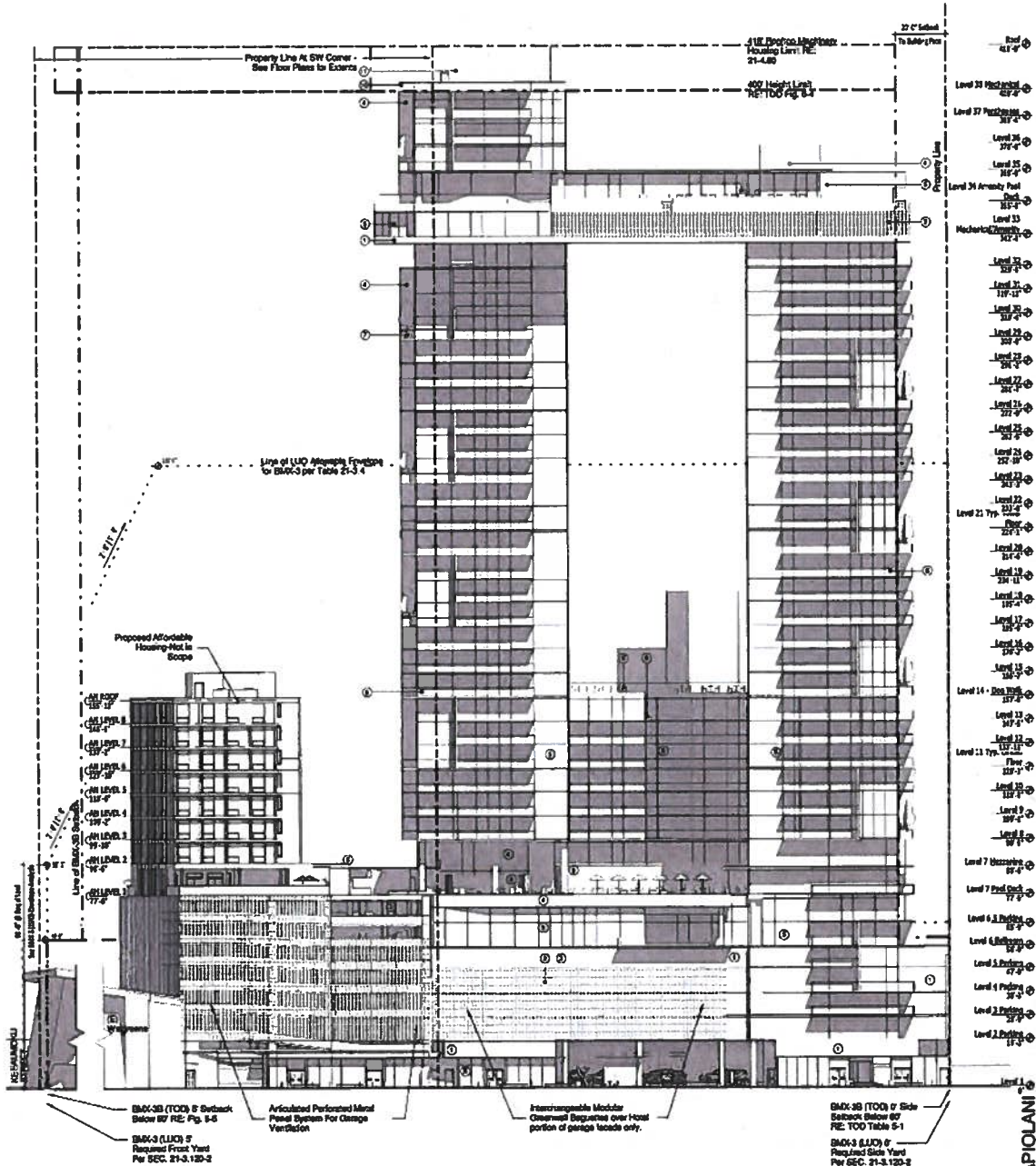
KAPIOLANI (SOUTH) ELEVATION 1" = 20'-0"
